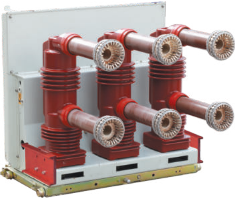
VCP-24
