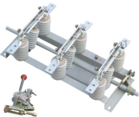
GN19-12
