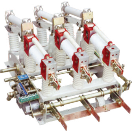
FZN21-12D/T630-20 FZRN21-12D/T125-31.5
