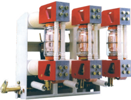
ZN28A-12 / ZN28-12
